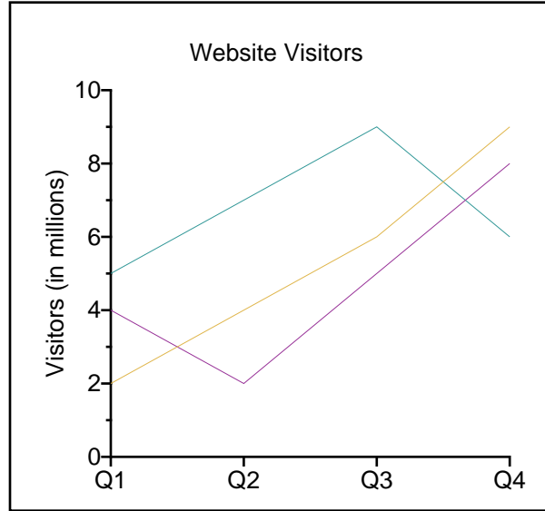
Line Chart
