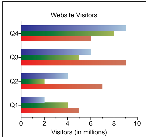
Bar Chart
