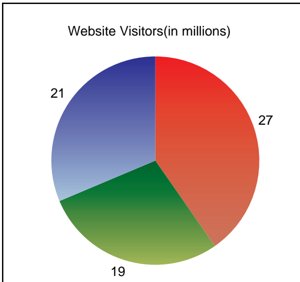
Pie Chart
